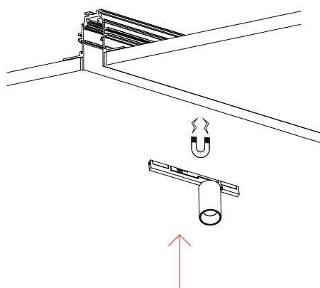
Recessed installation
