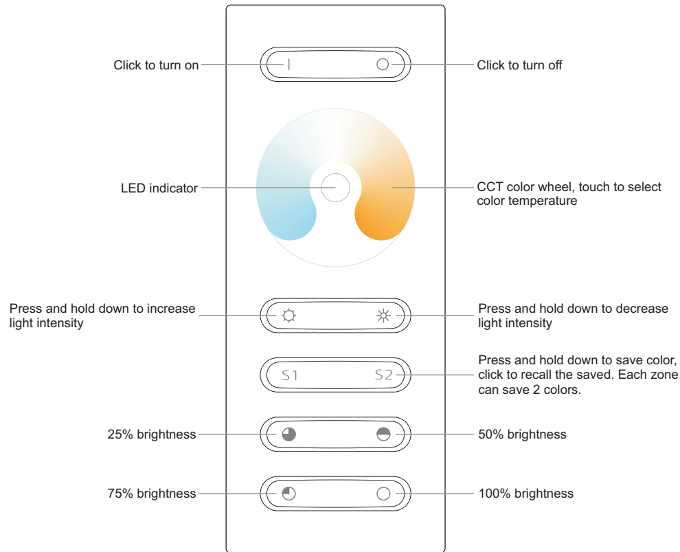
Front side
